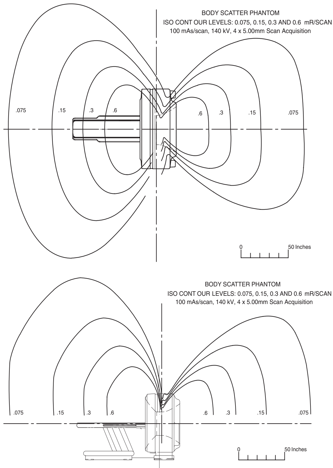
Figure 4-9 Typical Scatter Survey (Body Filter)
