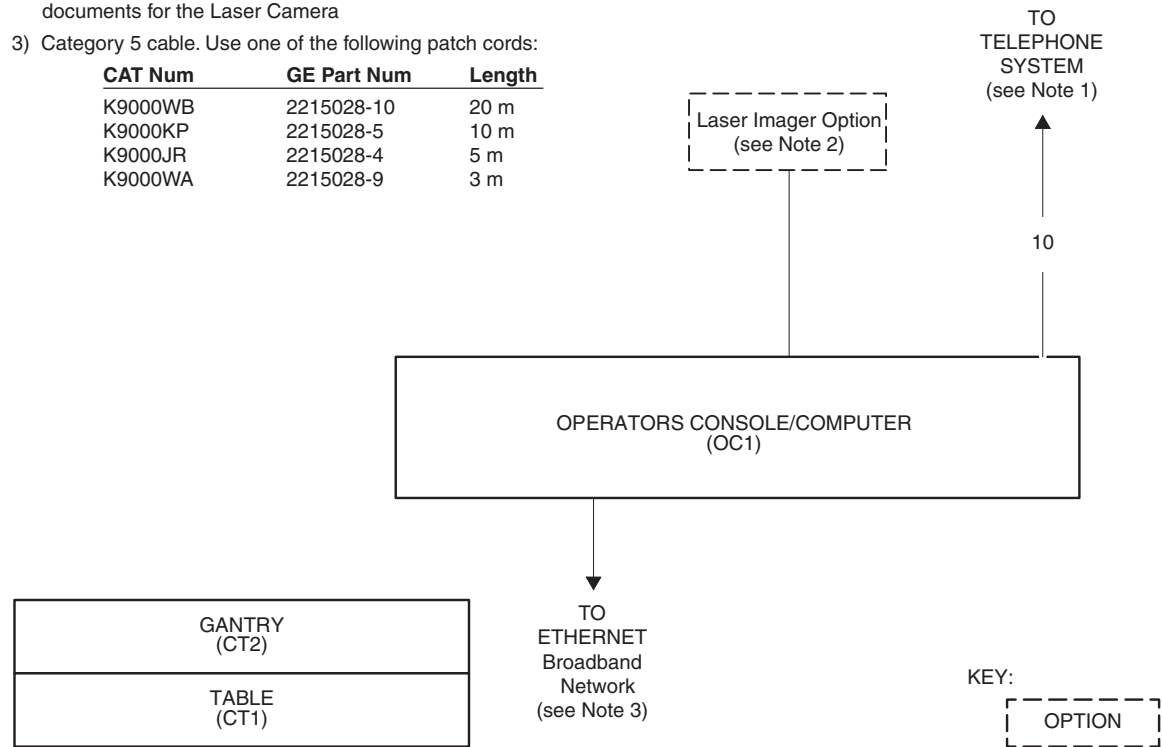
Figure 9-3 Interconnection Runs
