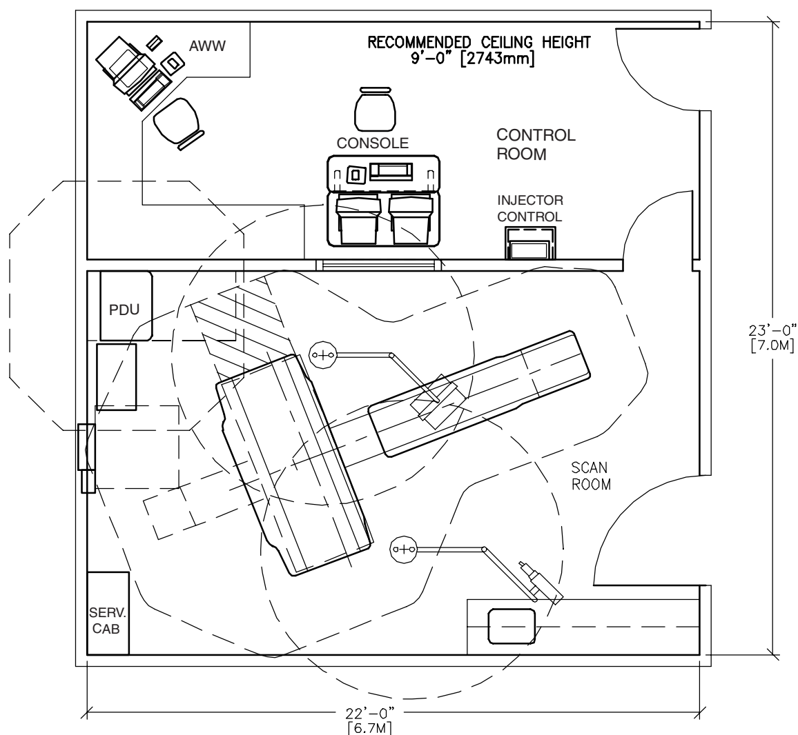
Figure 4-2 Standard Room Layout, with Injector Option
