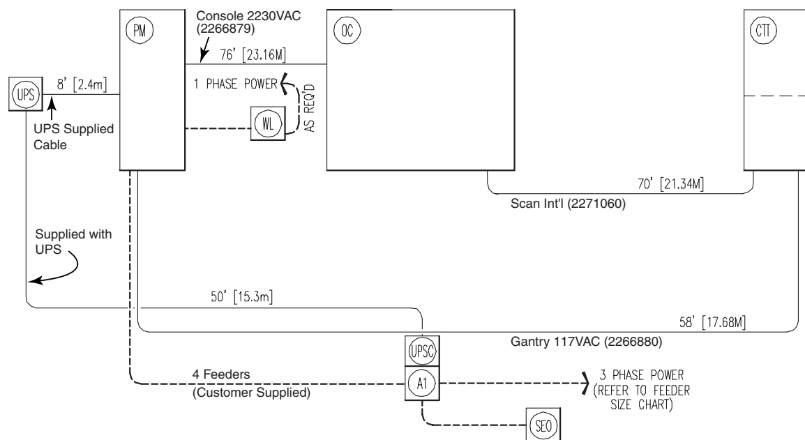
Figure 9-4 Typical UPS Interconnect
