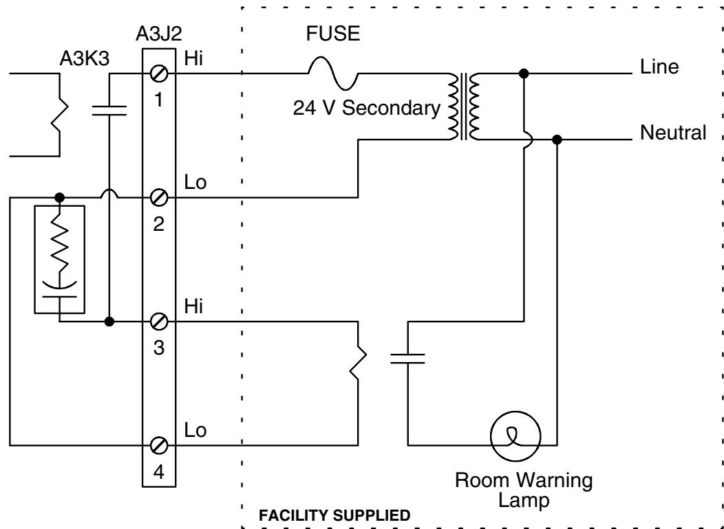
Figure 9-8 Typical Customer Supplied Scan Room – Warning Light Connection to PM
