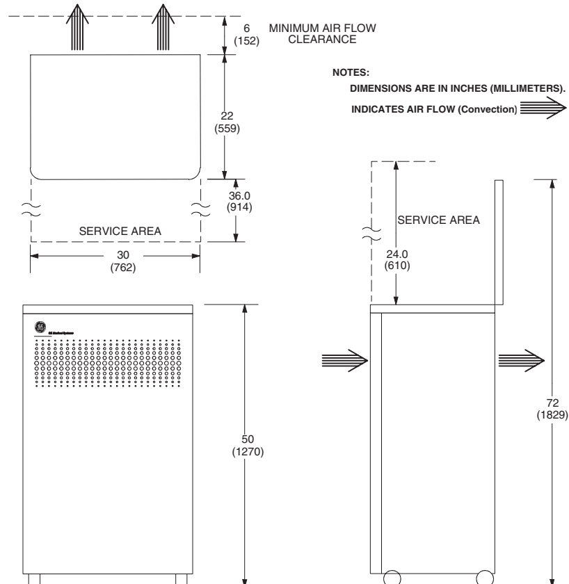
Figure 4-6 Compact Power Distribution Unit (PDU)
