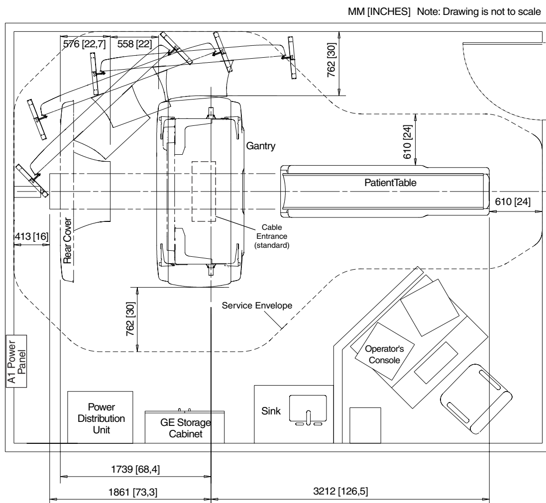
Figure 4-1 Sample Room Layout, Cover Removal Clearances
