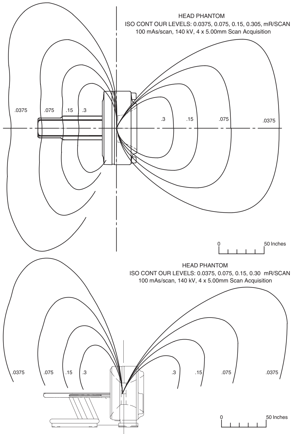
Figure 4-8 Typical Scatter Survey (Head Filter)
