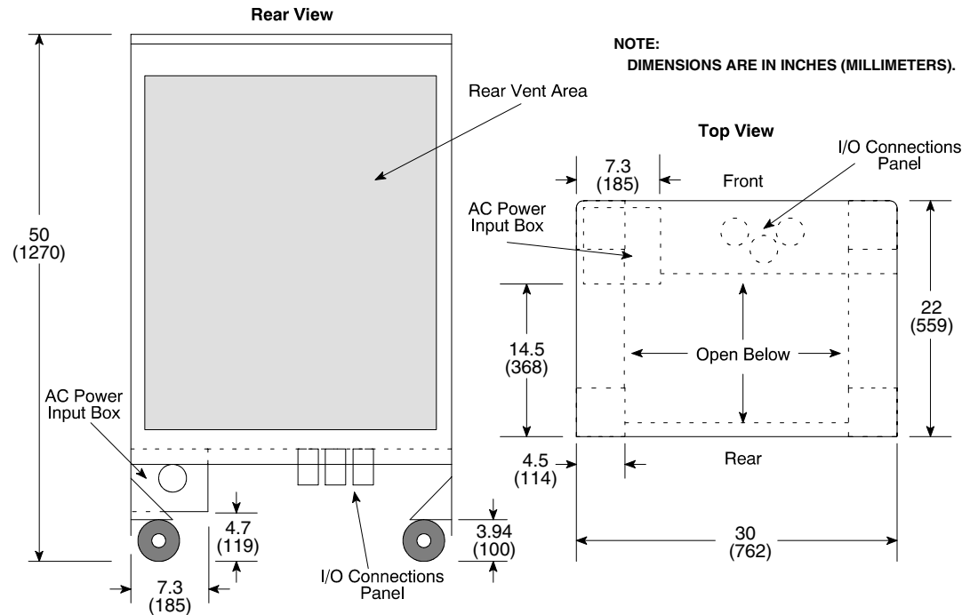
Figure 4-5 Compact Power Distribution Unit (PDU)
