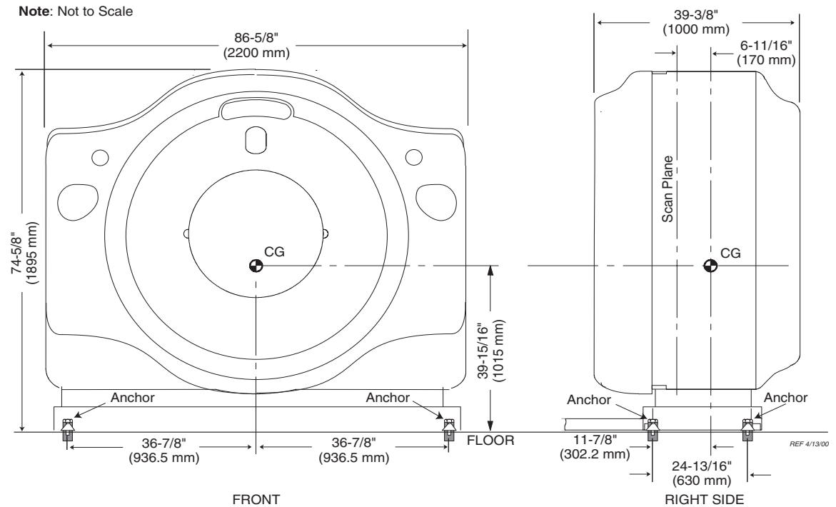
Figure 6-2 Gantry (CT2)
