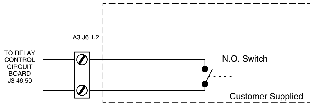
Figure 9-9 Typical Door Interlock
